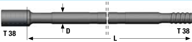
Flushing hole Ø 14.5 mm. Female end OD 56 mm
